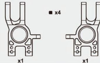
BB2134 4mm 7075 Front lower suspension mount (front)
