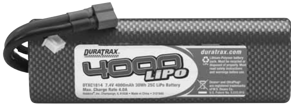
7.4V 4000mAh 25C LiPo Battery DTXC1814
