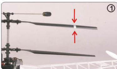
(1) 主旋翼旋转不在同一平面 Main blades don't rotate in one plane.
